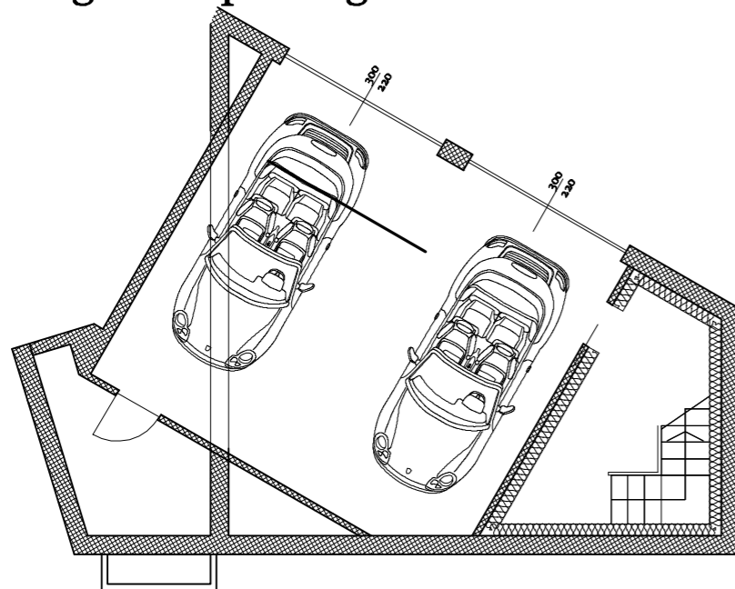
Underground parking
