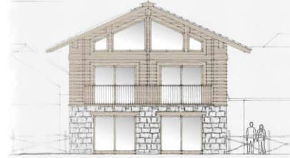
South elevation 1:100
