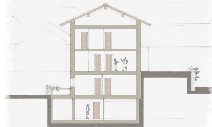
Section 1-1' 1:100
